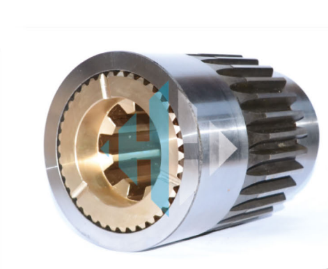
NAME: ROTATION BUSHING ASSY OEM: 152 493 48
